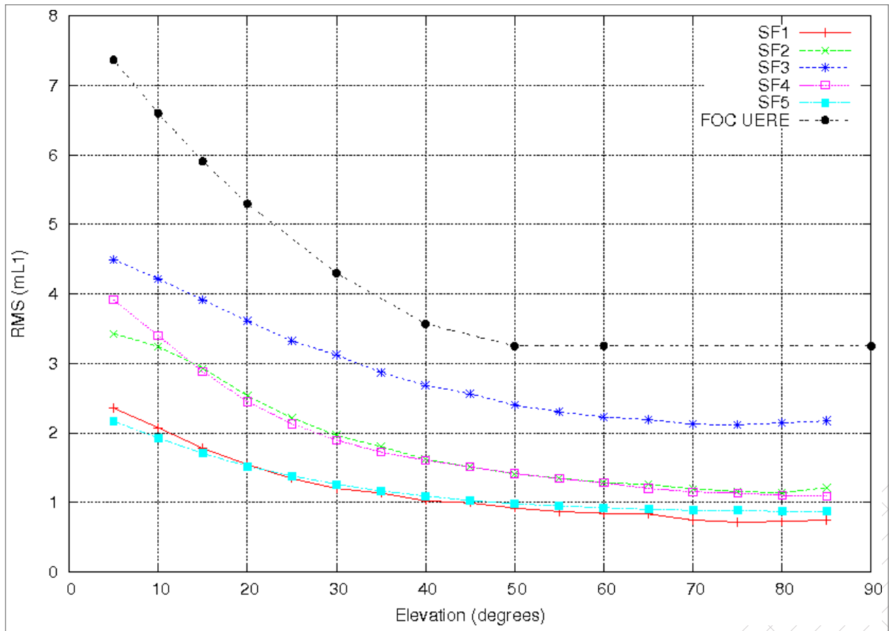
Figure 9. Residual single-frequency RMS error contribution to UERE after correction with single-frequency ionospheric algorithm [mL1]
