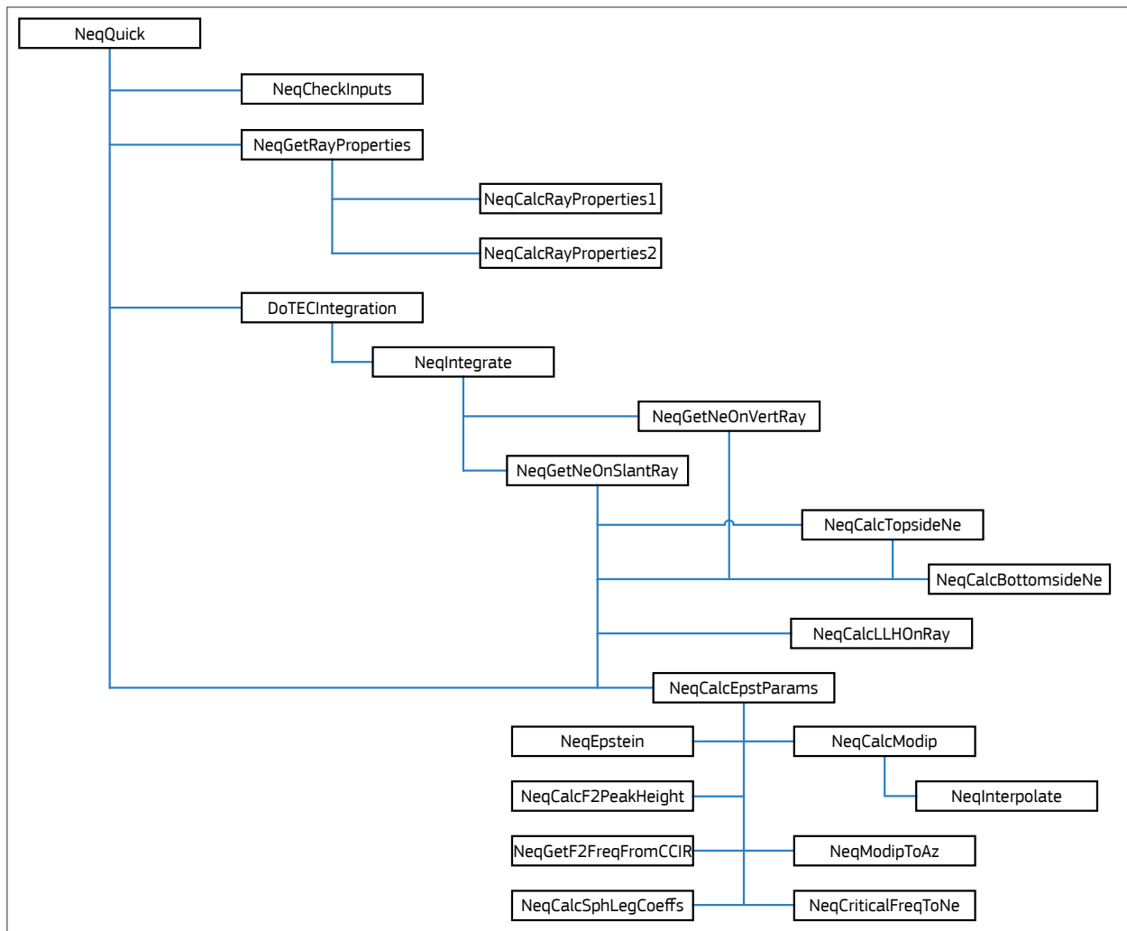
Figure 10. Overview of NeQuick Function Hierarchy
