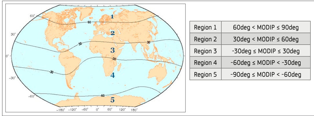
Figure 2. MODIP regions associated to different ionospheric characteristics
