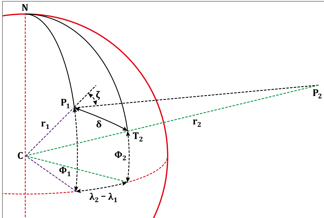
Figure 3. Geometry of zenith angle computation
