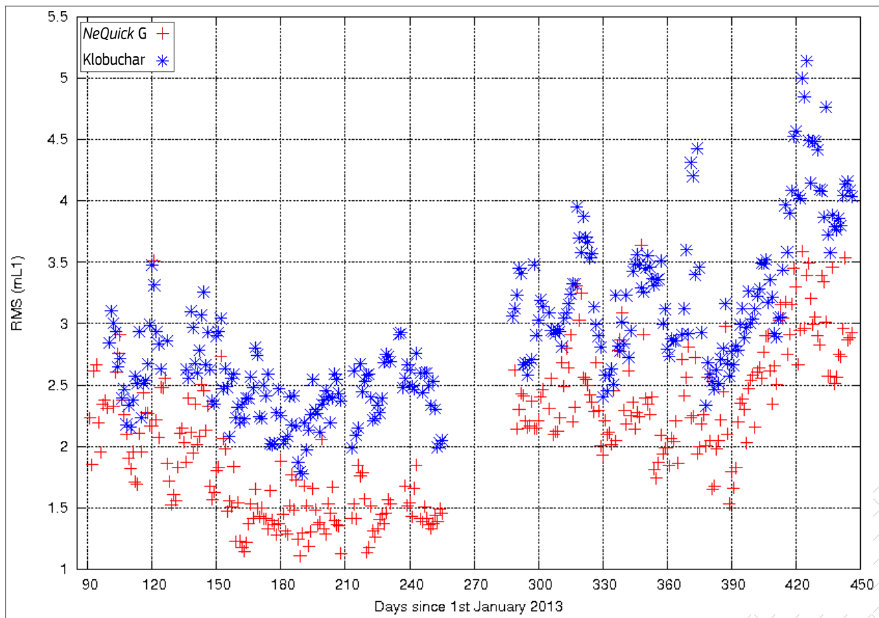
Figure 7. Global daily RMS ionospheric residual error [ m_{L1} ] after correction with Galileo NeQuick G (red) and GPS ICA (blue) from April 2013 to March 2014.
