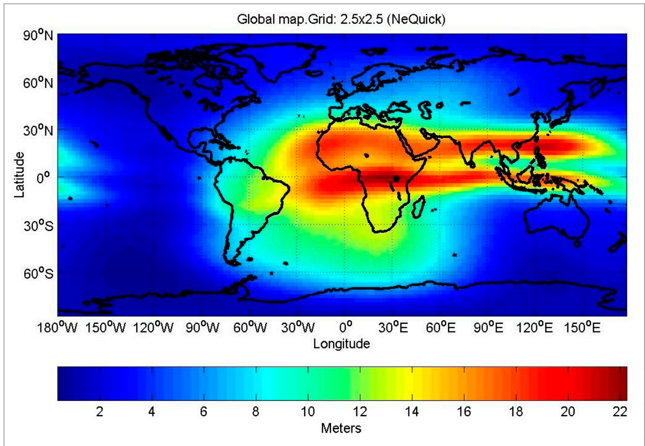
Figure 1. Example of a global VTEC map obtained with NeQuick
