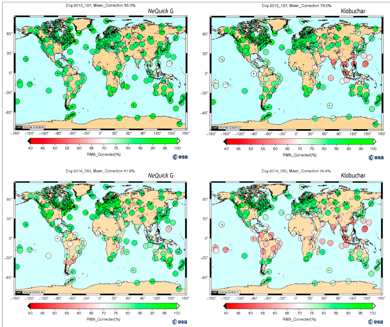
Figure 8. RMS correction capability (% with a lower bound of 20 TECU) of Galileo NeQuick G (left) and GPS ICA (right) correction models for day 127, 2013 (top) and day 80, 2014 (bottom)
