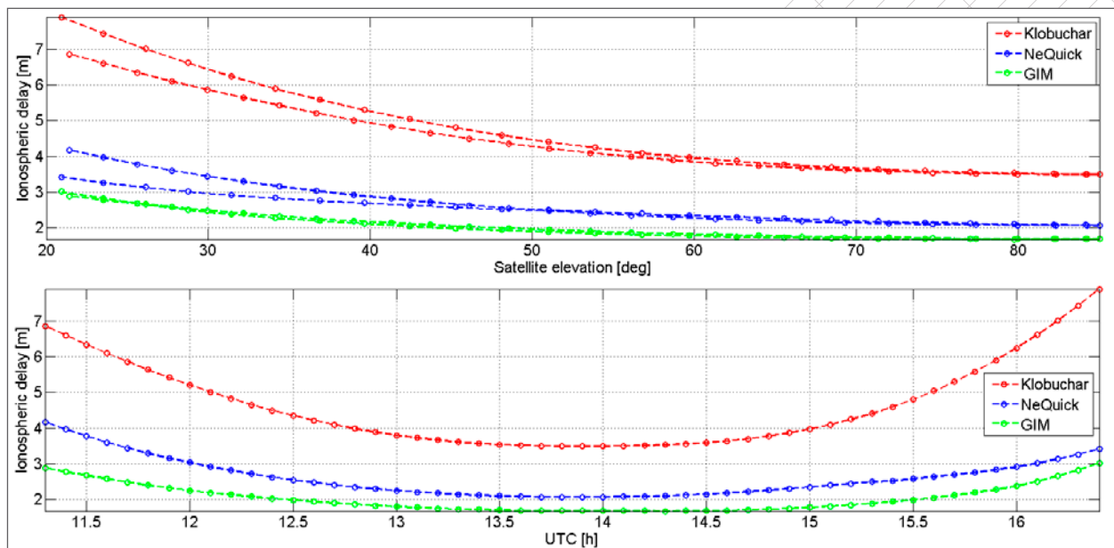
Figure 5. Ionospheric Delay vs. satellite elevation (upper) and of UTC (lower)
